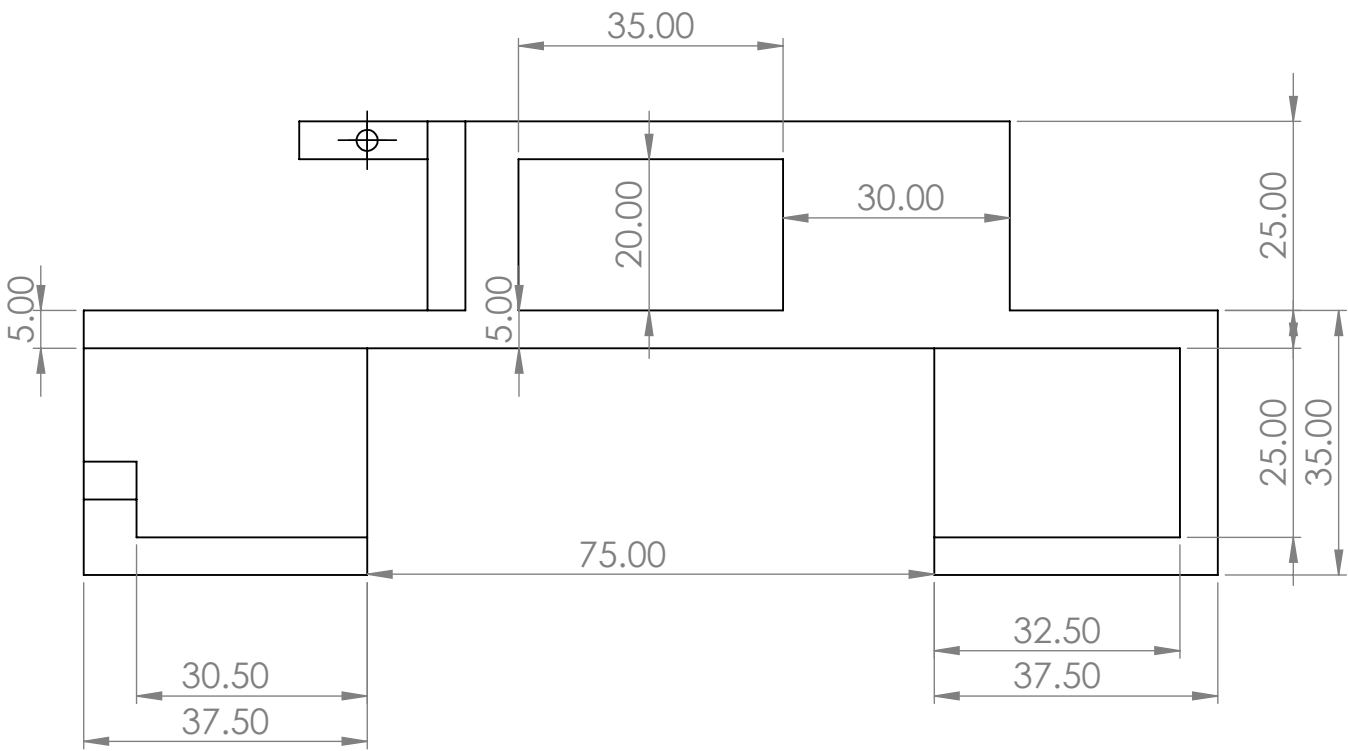
Vista Frontal
